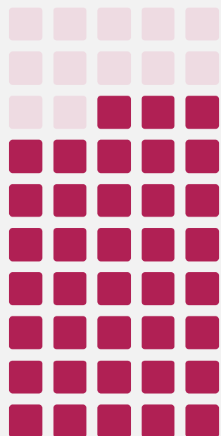
FEN standard
