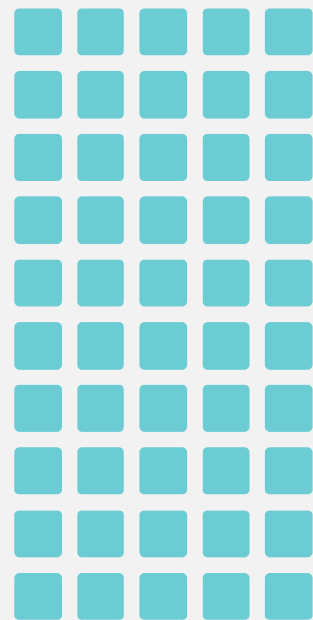
FEN s.operational
